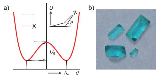
Figure 1. a) A schematic drawing of double-minimum potential U(\theta) for out-of-plane-bending deformation of four-membered-ring molecules. The observed values of \theta_0 and U_0 are 29^\circ , 515\text{ cm}^{-1} for \text{X}=\text{CH}_2 (cyclobutane); 28^\circ , 274\text{ cm}^{-1} for \text{X}=\text{S} (trimethylene sulfide); 0^\circ , 15\text{ cm}^{-1} for \text{X}=\text{O} (trimethylene oxide). [13] For \text{X}=\text{NH} (azetidine), the double-minimum potential becomes asymmetric ( U_0 \approx 440\text{ cm}^{-1} ). [13] b) Crystals of [(\text{CH}_2)_3\text{NH}_2][\text{Cu}(\text{HCOO})_3] .
